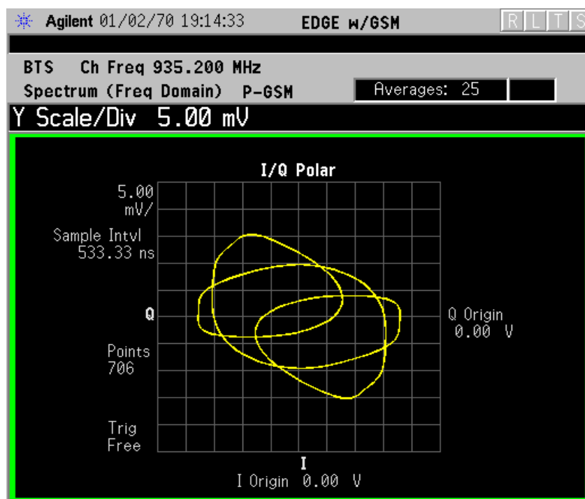
Figure 2-51 Spectrum Measurement - I/Q Polar View (for E4406A)
