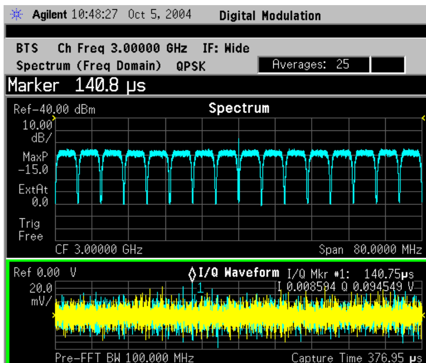
Figure 2-55 Spectrum Measurement - Spectrum Zoom View with Opt. 122–80 MHz Bandwidth Digitizer Hardware
