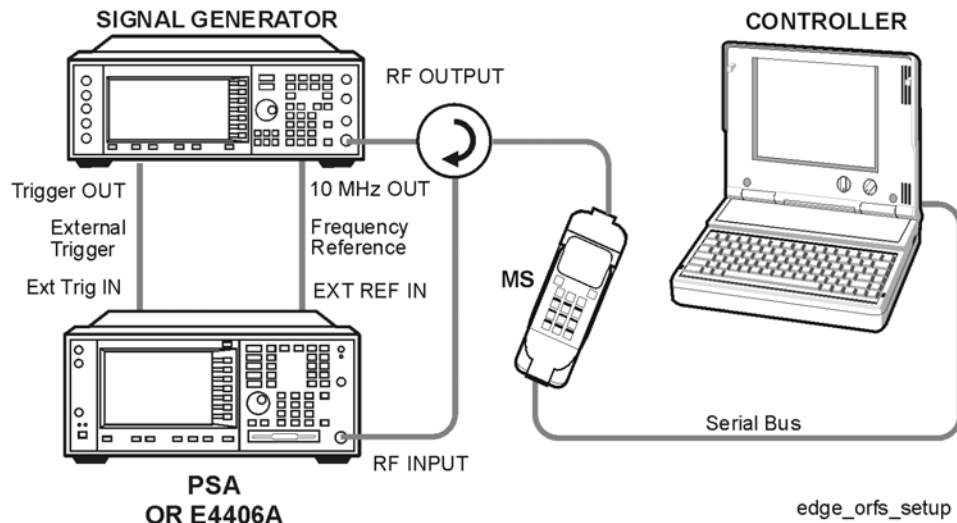
Figure 2-10 EDGE ORFS Measurement System
