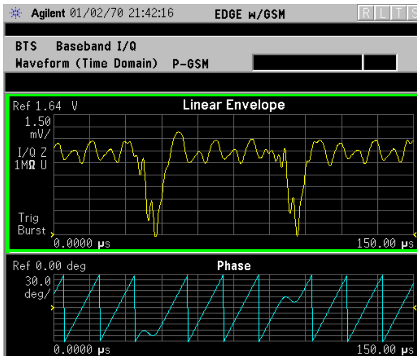
Figure 2-61 Waveform Measurement - Linear Envelope View
