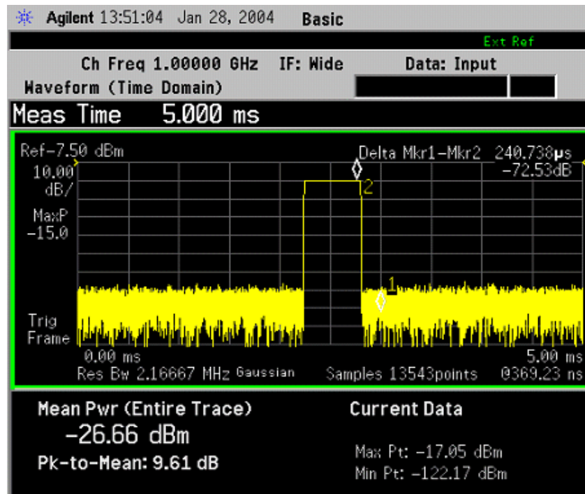
Figure 2-66 Waveform Measurement - RF Envelope View with Opt. 122–80 MHz Bandwidth Digitizer Hardware
