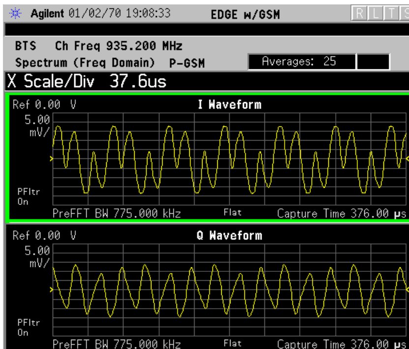
Figure 2-50 Spectrum Measurement - I and Q Waveform View (for E4406A)
