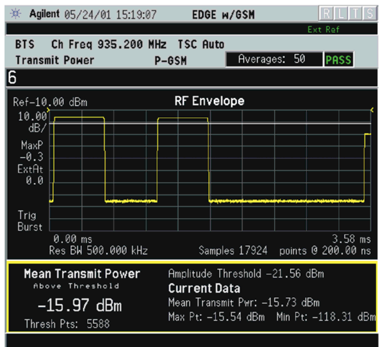
Figure 2-58 Transmit Power Result - Multiple Bursts
