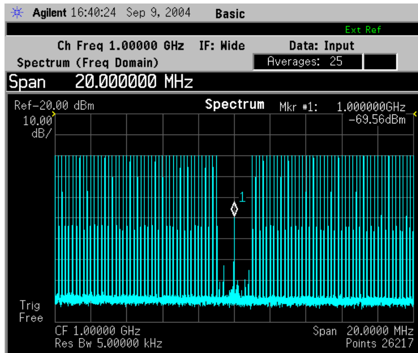
Figure 2-54 Spectrum Measurement - Spectrum View with Opt. 122– 80 MHz Bandwidth Digitizer Hardware
